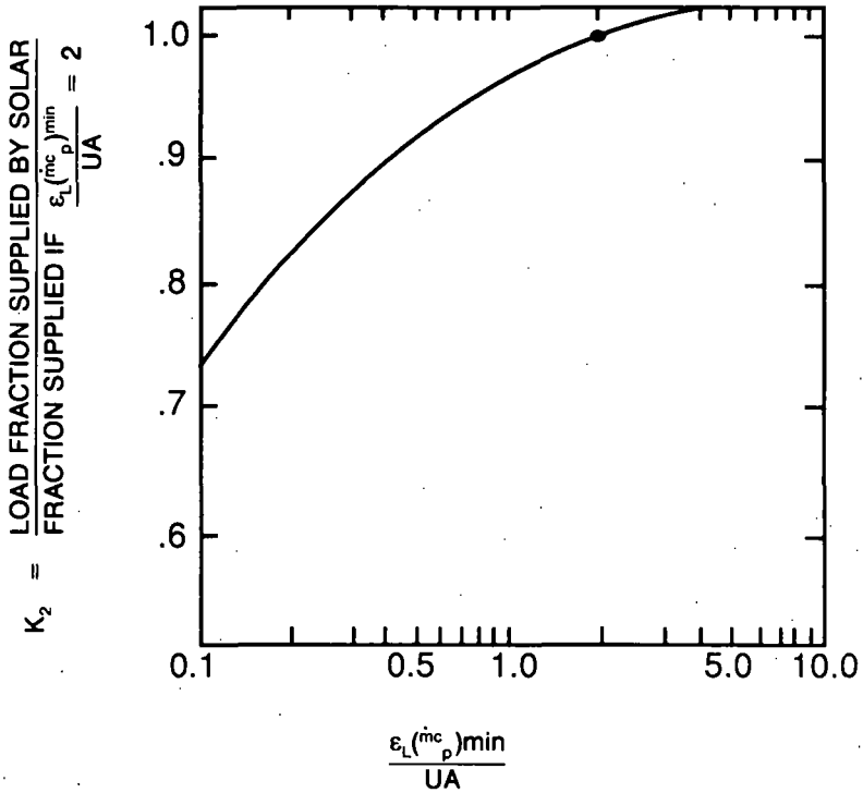
Correction factor ( K_2 ) for various values of \epsilon_L(\dot{m}c_p)_{\min}/UA .
