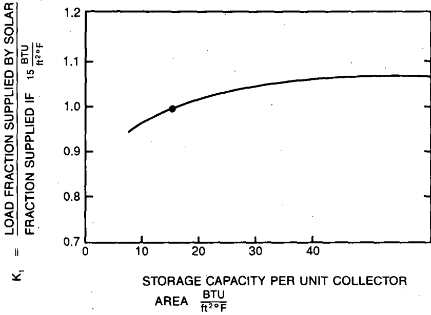
Correction factor ( K_1 ) for storage capacities other than 15 BTU/ft 2 °F.
