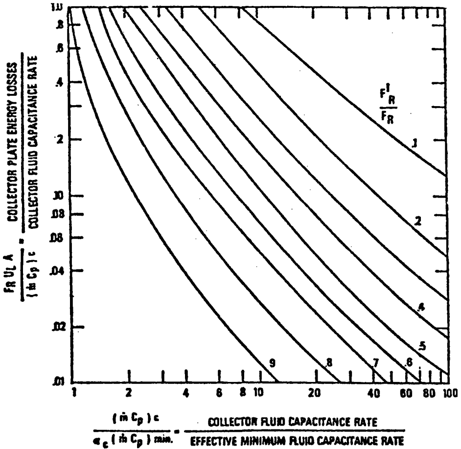
F_R' / F_R as a function of F_R U_L A / (\dot{m} C_p)_c and (\dot{m} C_p)_c / \epsilon_L (\dot{m} E_p)_{min} .
