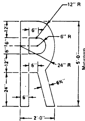
PAVEMENT MARKINGS MINNESOTA DEPARTMENT OF TRANSPORTATION
