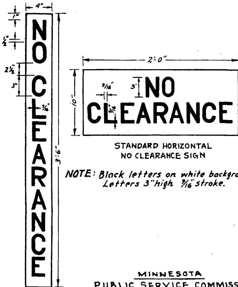
STANDARD VERTICAL NO CLEARANCE SIGN
