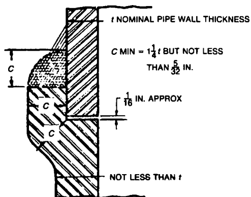
5230.1240 FIGURE 7: MINIMUM DIMENSIONS REQUIRED FOR SOCKET WELD FITTINGS.
