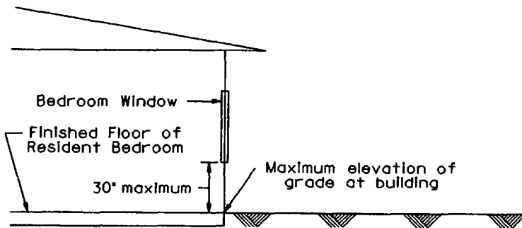
RESIDENT BEDROOM - ROOM AT GRADE
